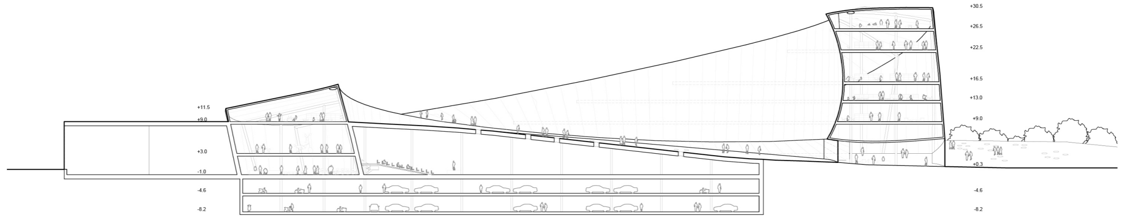
Section 1-1
